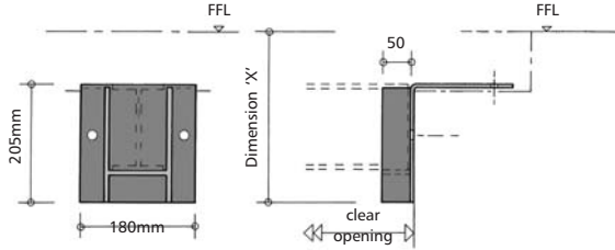
BEAM BRACKET NO. 2
